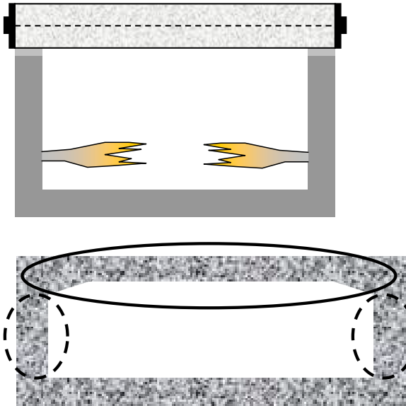
Figure 2.4.2: horizontal test, representing a tunnel ceiling but also conservative for the walls
