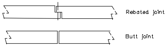
Figure 3.2.2: Joint types
