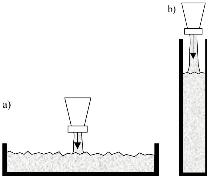
Figure 2.1.1: specimens cast in the correct position; a) wall or ceiling; b) wall
