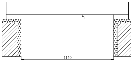
B. Cross section I-I: slab with board insulation material
